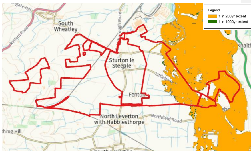
Figure 5.9: Modelled undefended tidal dominated flood extent (2023 Jacobs Tidal Trent model)
